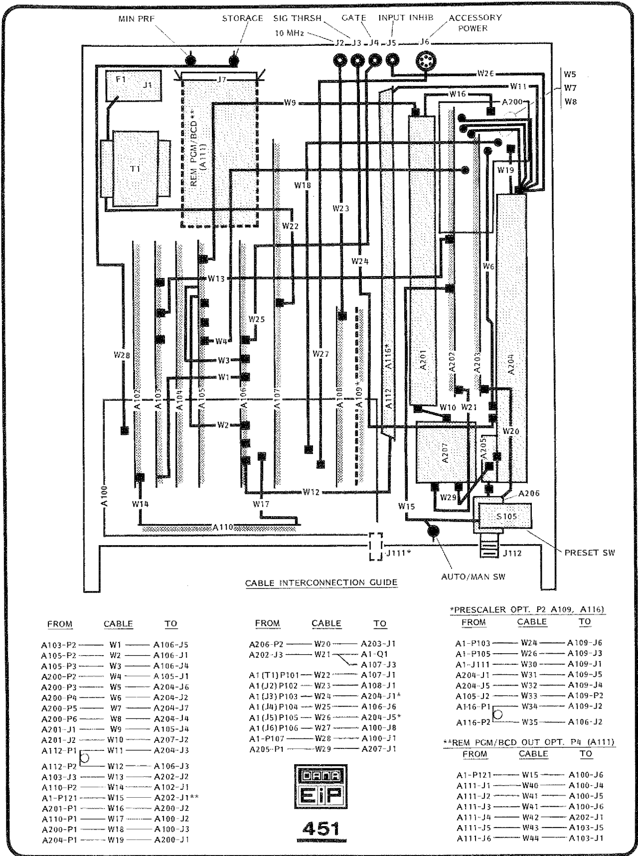
FIGURE 9-1 ASSEMBLY LOCATOR CABLE INTERCONNECTIONS
