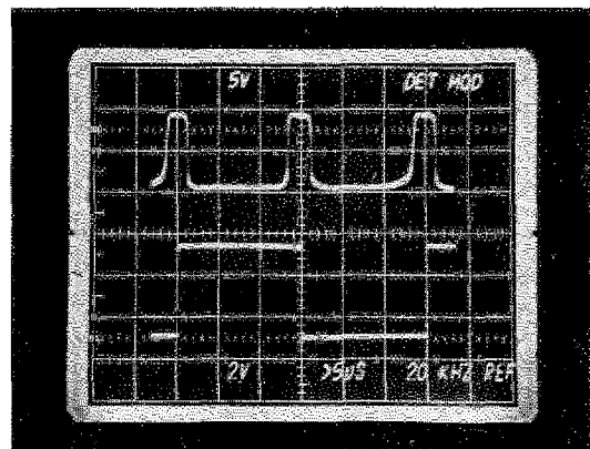
FIGURE 6-2 DETECTED MOD/20 kHz REFERENCE PULSE TIMING
