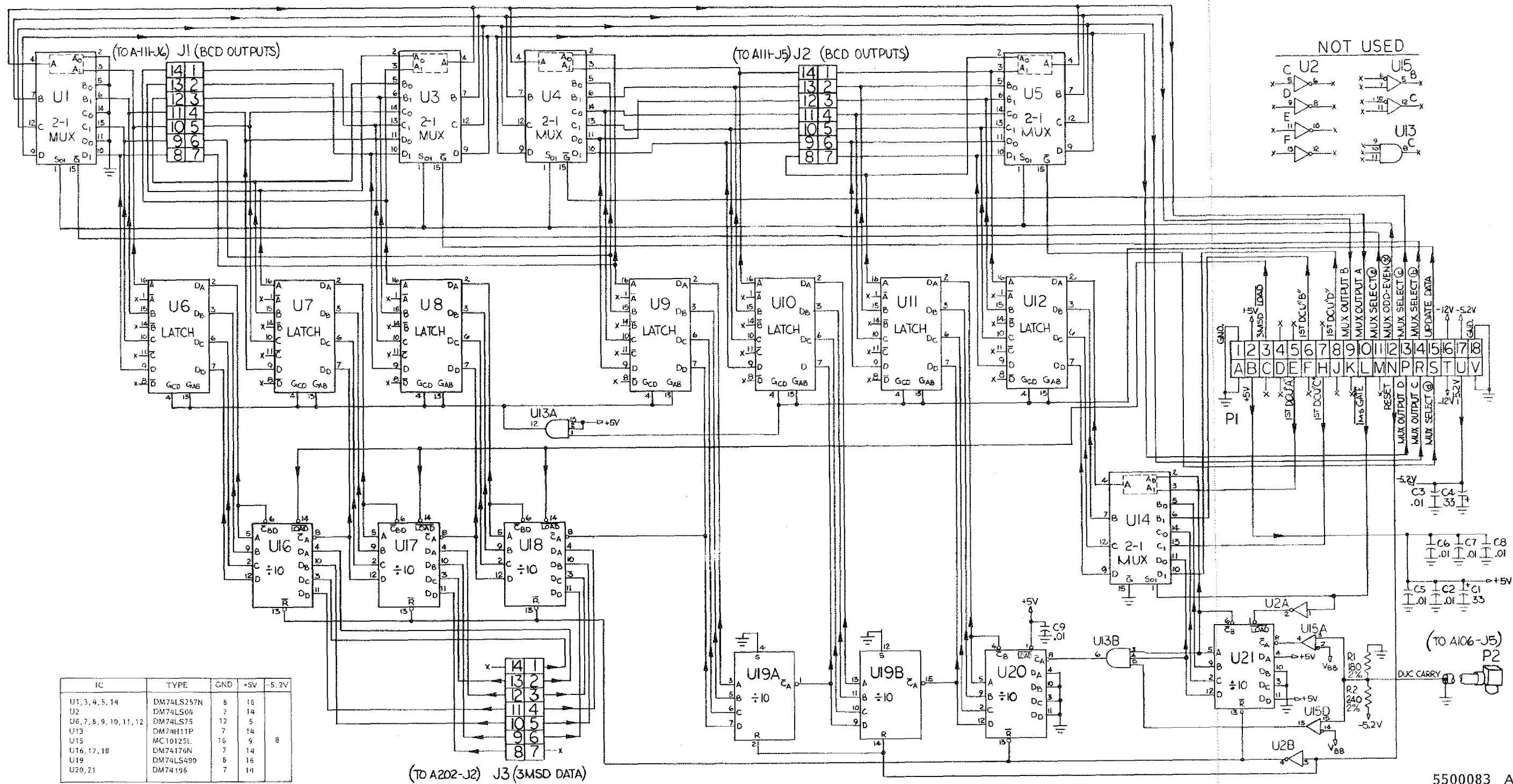
FIGURE 9-5B SCHEMATIC DIAGRAM COUNT CHAIN (A103)
