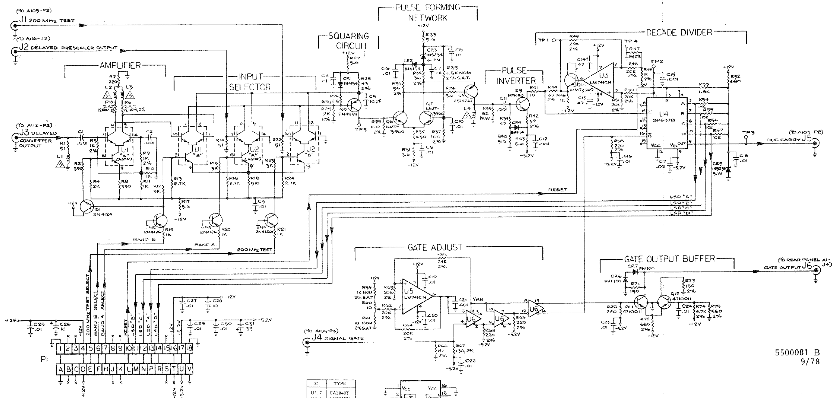
FIGURE 9-8B SCHEMATIC DIAGRAM HIGH FREQUENCY (A106)
