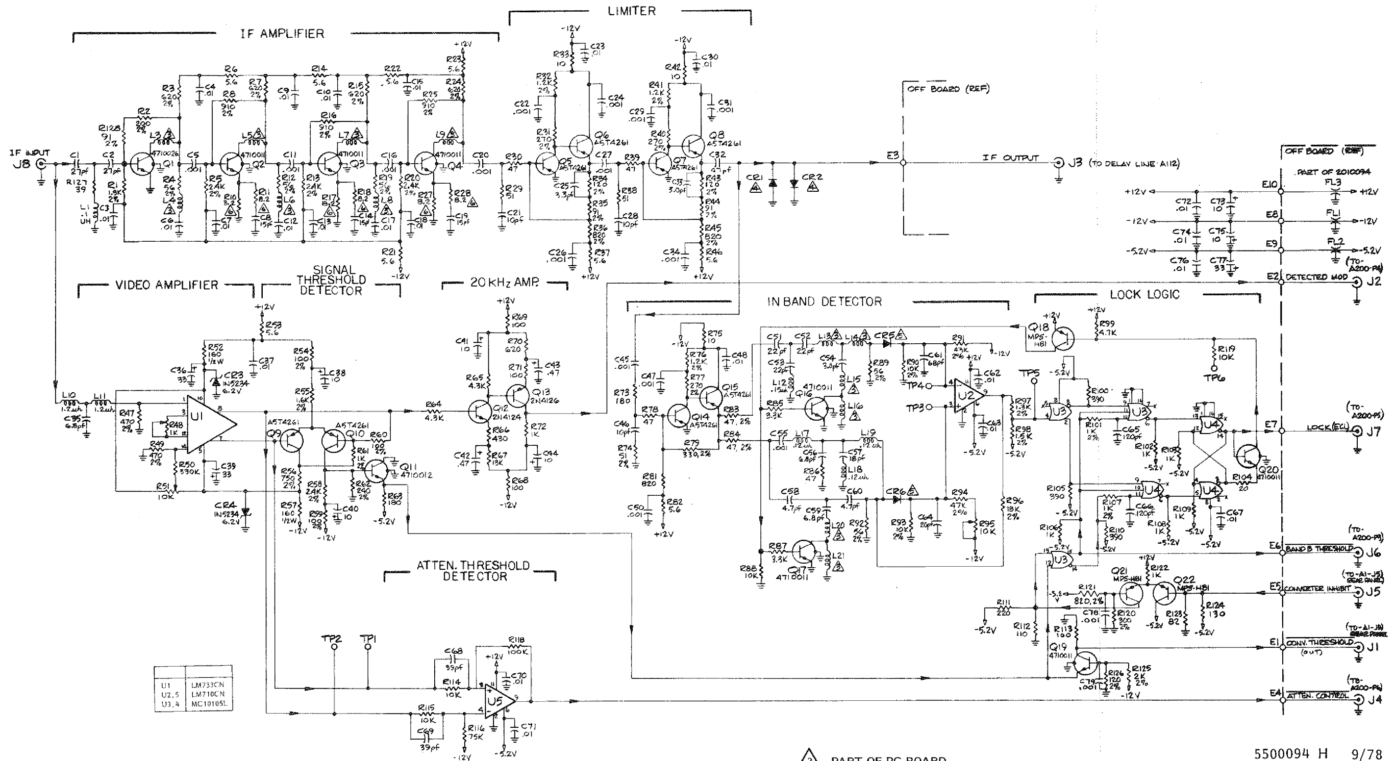
FIGURE 9-16B SCHEMATIC DIAGRAM IF PROCESSOR (A204)
